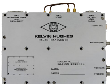
SharpEye™ transceiver located in upmast turning unit housing
